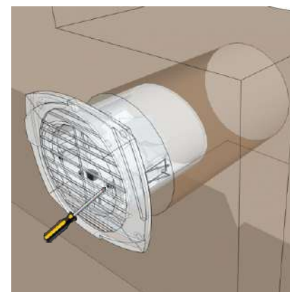
Brzim zatezanjem žabica u odgovarajući otvor Fast installation by tightening hooks into matching hole
