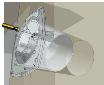
Brzim zatezanjem žabica u odgovarajući otvor Fast installation by tightening hooks into matching hole
