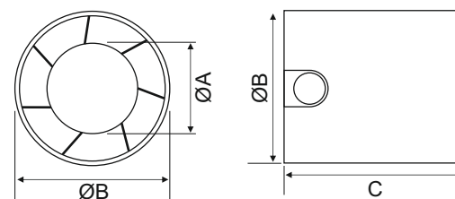
Dimenzije (mm) / Dimensions (mm)
